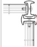
MESH FIXING CORNER POST 90°
